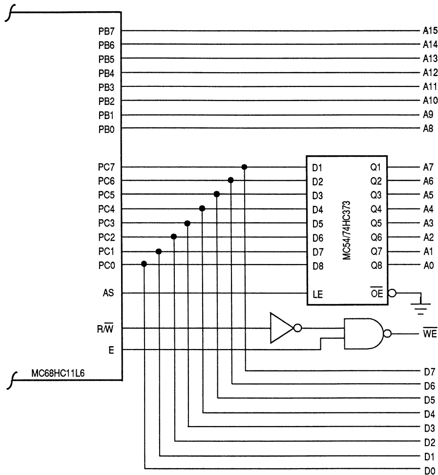
Address/Data Demultiplexing
