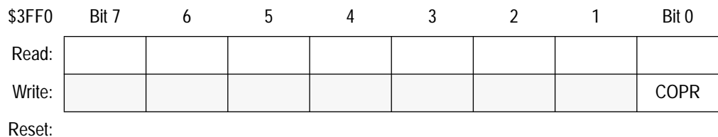
Figure 5-3. COP Watchdog Timer Location Register (COPR)
