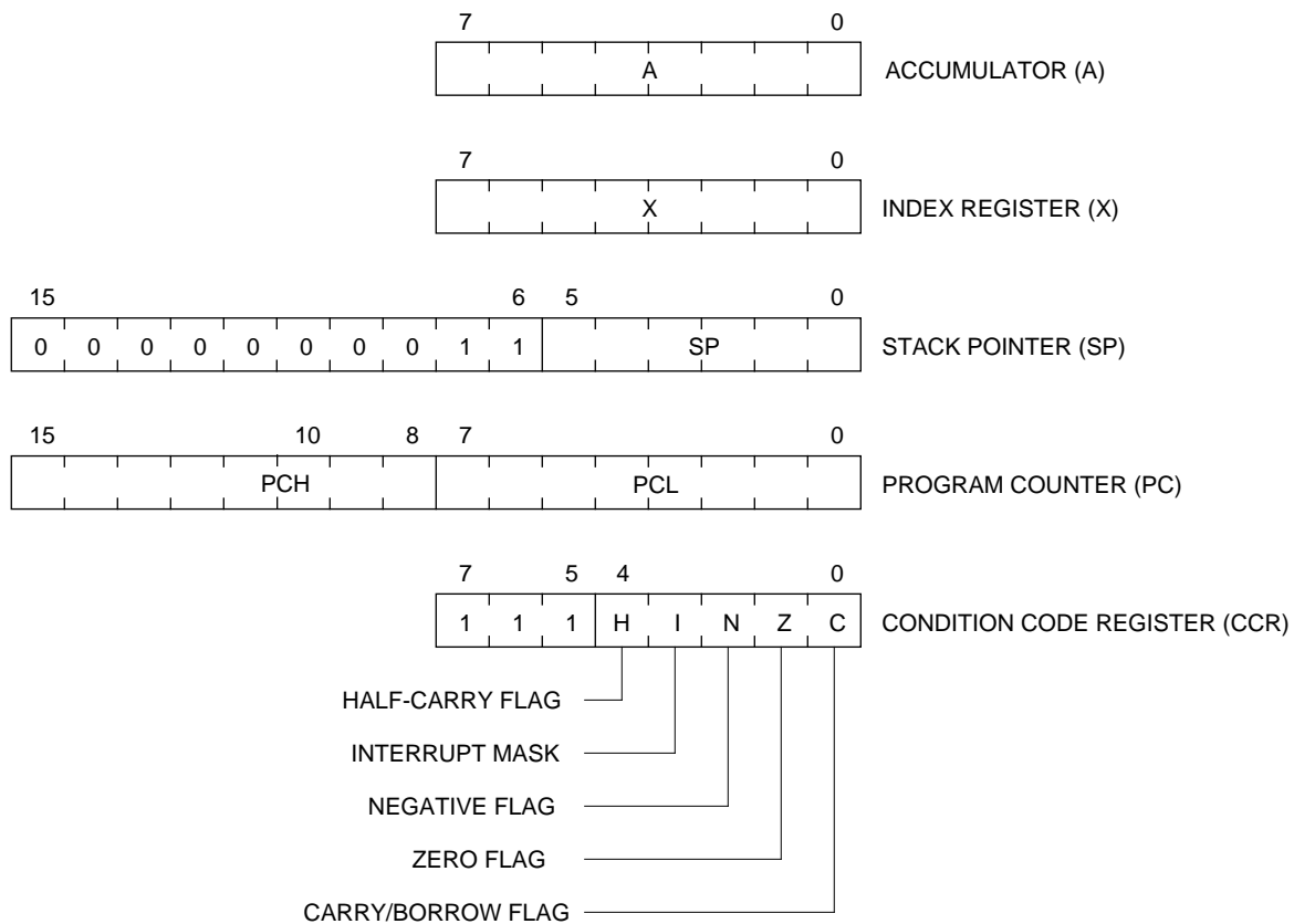
Figure 3-1. Programming Model
