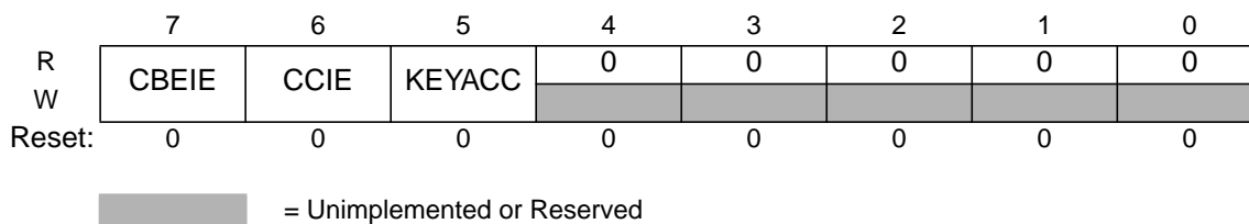
Figure 3-5 Flash Configuration Register (FCNFG)
